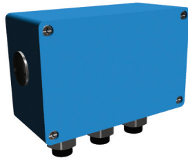
Small auxiliary aluminum terminal box for motor sizes 280–500 (variant codes 418, 568, 380, 569) The size of terminal box ordered with these codes depends on the number of accessories ordered. 80 x 125 mm, max 12 strips. Earthing size M4
