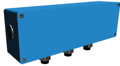
Large auxiliary aluminum terminal box for motor sizes 280–500. The size of terminal box ordered with these codes depends on the number of accessories ordered. 80 x 250 mm, max 30 strips. Earthing size M4
